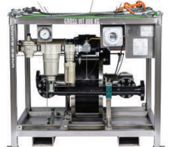
P6 High Pressure Fluid Transfer Pumps & Low Pressure Fluid Transfer Pumps. Hydraulic Flushing & Parti- cle Counting Systems.
