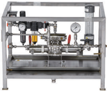
P1 Series Low Volume Chemical Injection Skids.
